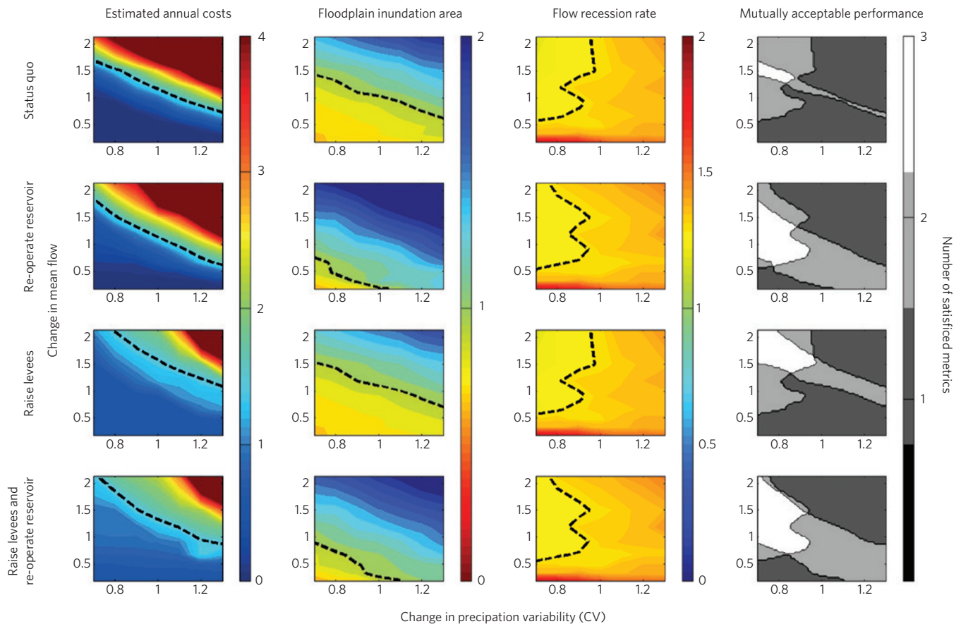
Figure 4 | Three lowa River system performance indicators mapped in a variable future climate space defined by change in annual precipitation variability and mean annual flow for each of 4 management actions (rows). The estimated annual costs and the floodplain inundation area are as in Fig. 3. The third column is the flow recession rate indicator, with values exceeding the threshold of +30% of historical, unregulated inflow recession rates (shown on colour scale at 1.3) being unacceptable (to the left of the dashed line). Mutually overlapping performance for all combinations of the three indicators (one engineering and two ecological) is shown in the fourth column for each of four management actions.
